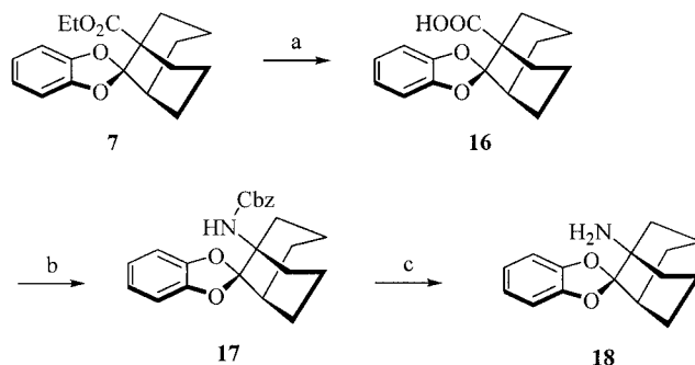
Scheme 4. Synthesis of subunits: a) 1. KO t Bu, THF, H 2 O, 0 °C, then reflux, 16 h, 2. 0 °C, conc. HCl, 88%. b) 1. Toluene or benzene, DMF, DPPA, NEt 3 , 0 °C, 30 min., then reflux, 3 h, 2. BnOH, reflux, 24–36 h, 92%. c) Pd(OH) 2 /C, H 2 , THF, room temp., 48 h, quantitative.
