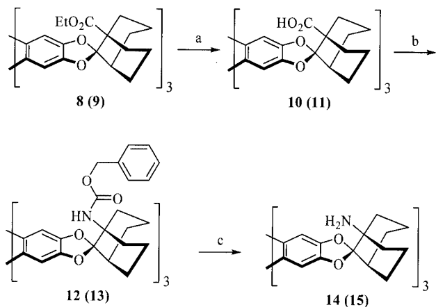
Scheme 3. Synthesis of the modified all-syn derivatives ( anti,anti,syn compounds): a) 1. KO t Bu, THF, H 2 O, 0 °C, then reflux, 16 h, 2. 0 °C, conc. HCl, 10 : 87% ( 11 : 92%). b) 1. Benzene, DMF, DPPA, NEt 3 , 0 °C, 30 min., then reflux, 4 h, 2. BnOH, reflux, 36 h, 12 : 81% ( 13 : 85%), c) Pd(OH) 2 /C, H 2 , THF, room temp., 48 h, 14 : 99% ( 15 : 99%).
