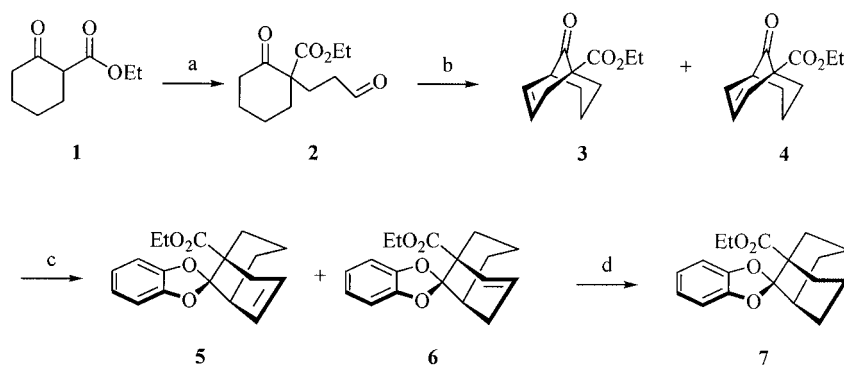
Scheme 1. Synthesis of bicyclic spiroketal 7 . a) acrolein, \text{NEt}_3 , DMF, room temp., 16 h, 92%. b) \text{H}_2\text{SO}_4 , -10\text{ }^\circ\text{C} \rightarrow \text{room temp.} , 22 h, 77%. c) catechol, p\text{TsOH} , toluene, Dean–Stark trap, 22 h, 84%. d) \text{Pd/C} , \text{H}_2 (1 atm), THF, 40 h, 100%.
