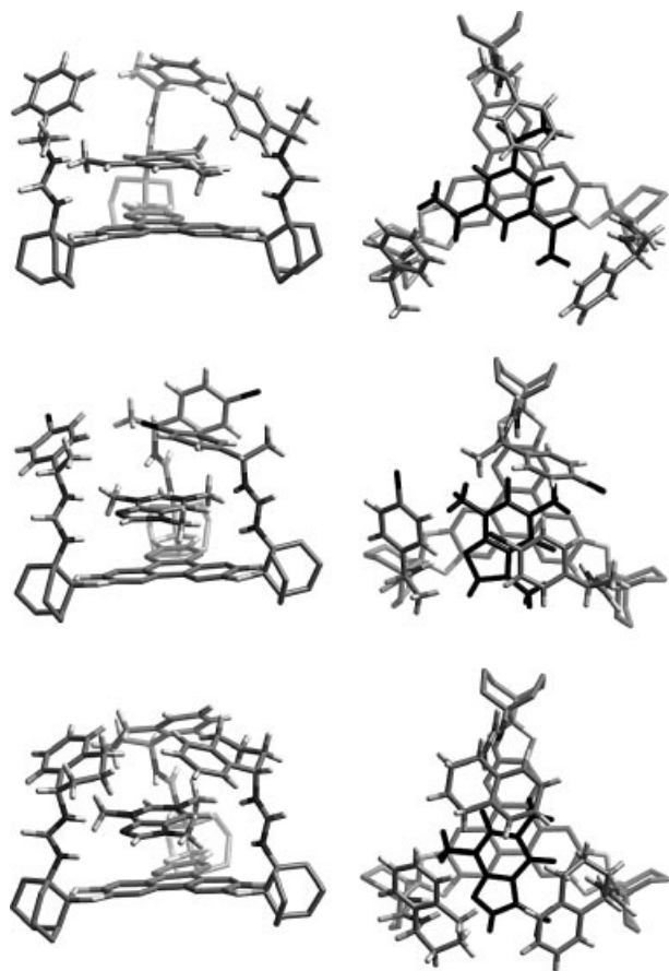
Figure 3. Molecular structures of triacetyl benzene with 19a (top) and caffeine complexes of 19b (middle) and 19c (bottom). Left column: side view of the complexes. Right column: top view.
