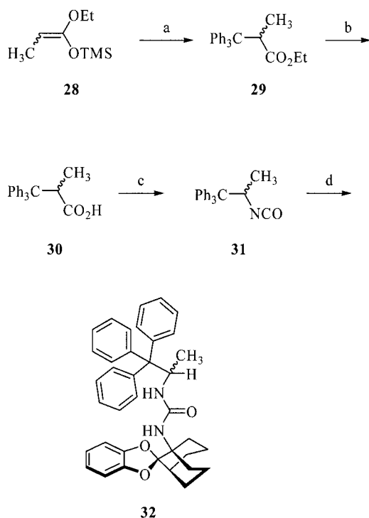
Scheme 5. Synthesis of trityl-substituted receptor subunit 32 : a) Et 2 O, Ph 3 CBF 4 , 0 °C → room temp., 1 h, 60%. b) KOH, EtOH, H 2 O, reflux, 64 h, 67%. c) Acetone, DPPA, 0 °C, 45 min., then toluene, reflux, 3 h. d) NEt 3 , 18 , 0 °C → room temp., 14 d, 89%.
