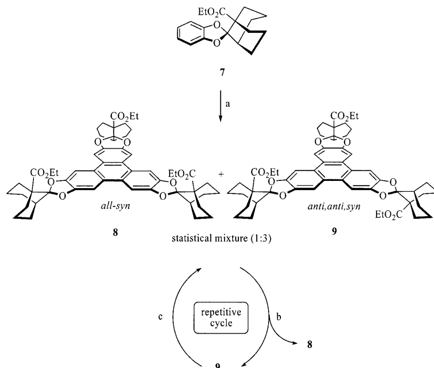
Scheme 2. Access to all-syn triester 8 : a) Pt electrodes, 20 °C, 0.1 M NBu 4 BF 4 in H 3 CCN, 0.45 A·cm -2 , 3.1 F, up to 90%. b) Crystallization from toluene/ethanol (4:1). c) 1. ClCH 2 CH 2 Cl, reflux, 2. F 3 CSO 3 H, reflux, 15 min., 3. NEt 3 , then 0 °C.
