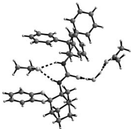
Figure 2. Crystal structure of 32 .
